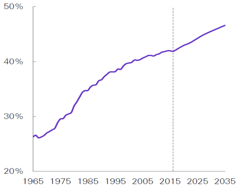
Share of power sector in primary energy consumption
